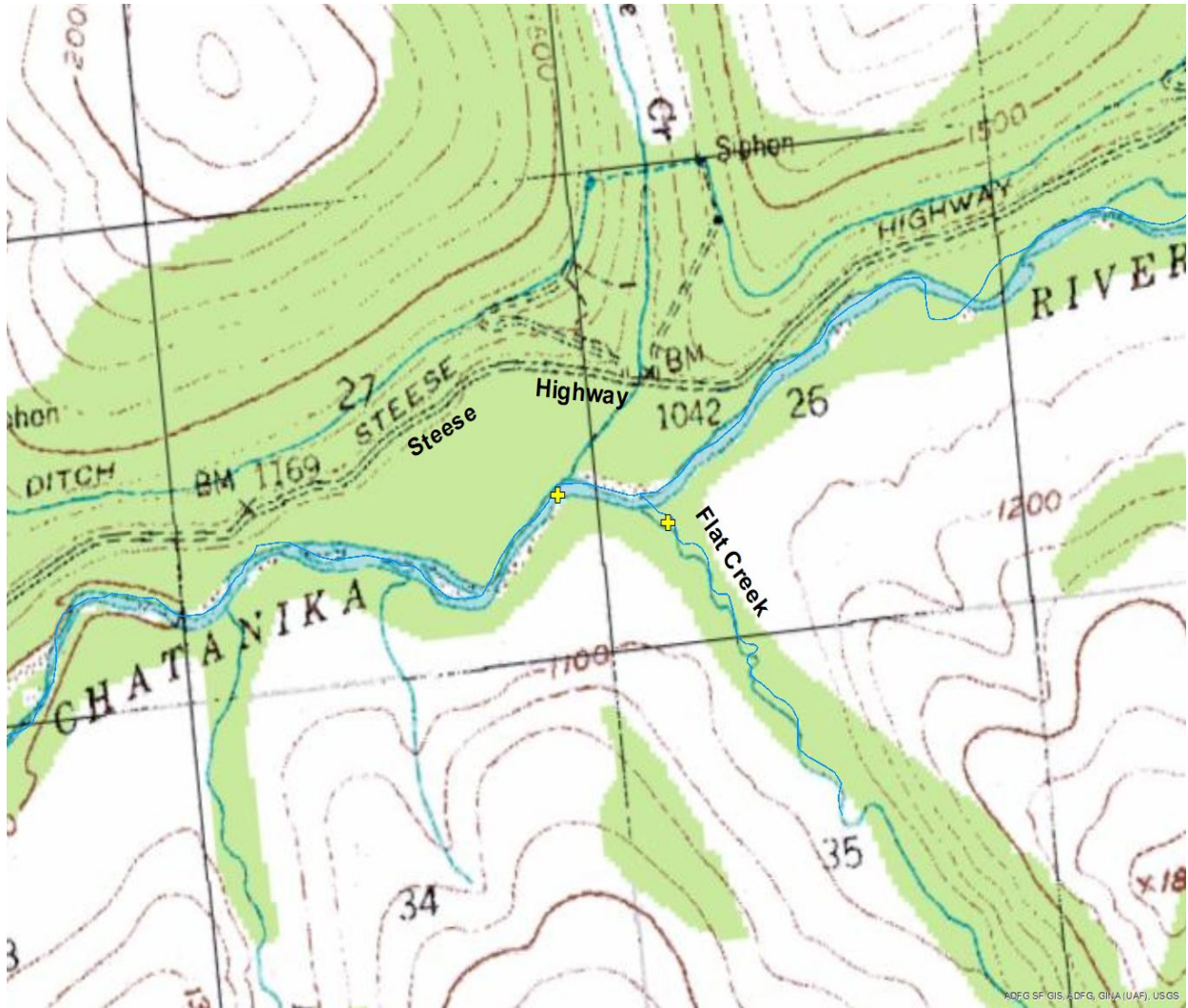
Figure 1. Upper Chatanika River and Flat Creek crossing points (yellow +).
